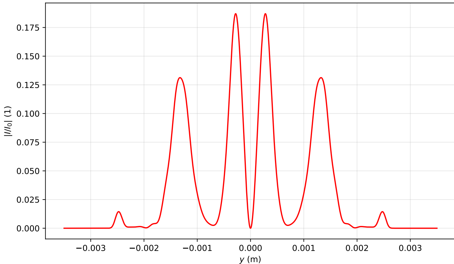
Intensity profile I(x=0, y, z=2.070)/I_0 , \text{Pin}=9.0\text{Pcr} , artificial time
